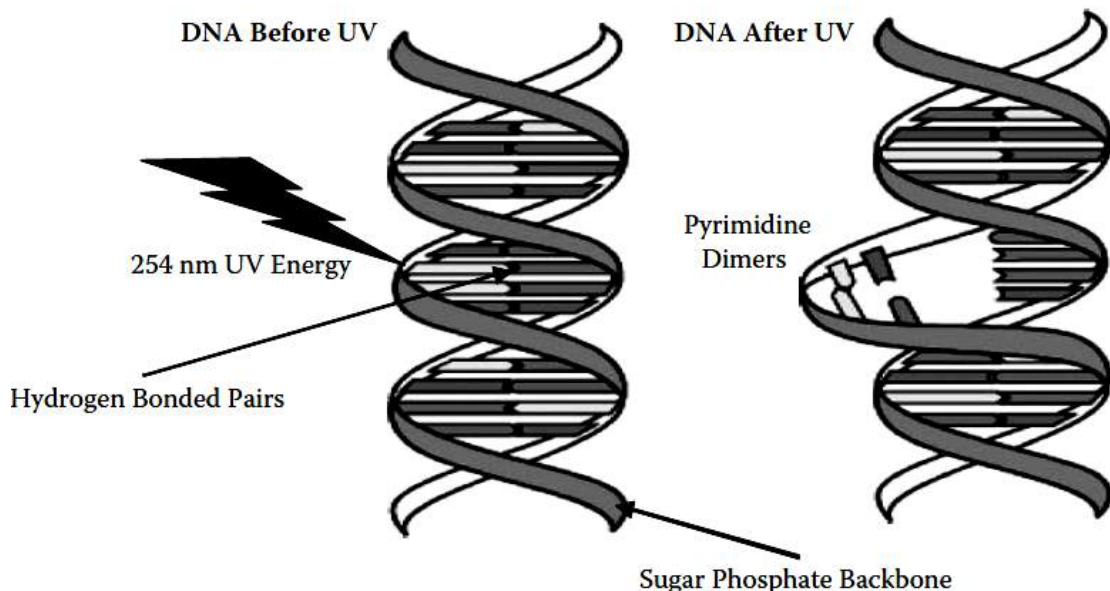
Figure 2 Structure of DNA before and after UV irradiation [17]
